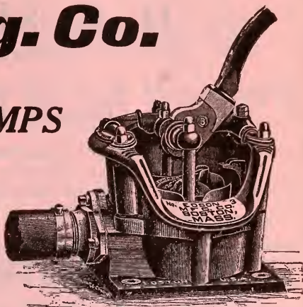
Edson's Diaphragm Pumps with Suction Hose to Let
