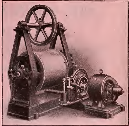
Payne Direct Connected Elevator Machine
