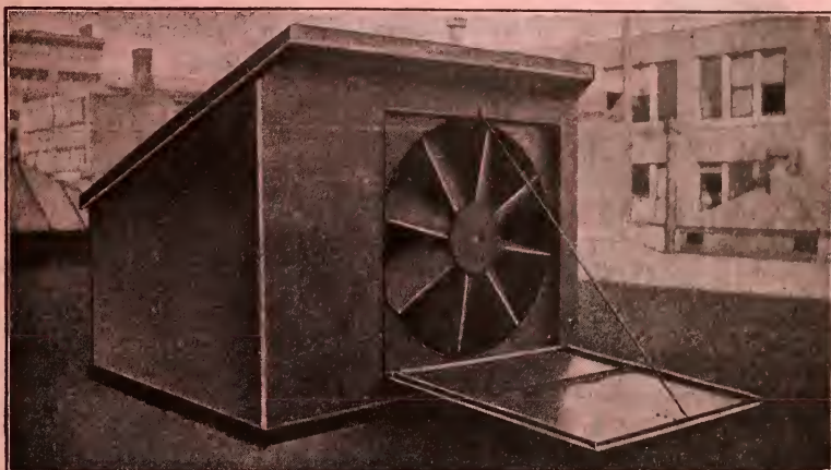
One of Our 48 Vent Apparatus Installed at Manhattan Market Co., Cambridge, Mass., 1915
