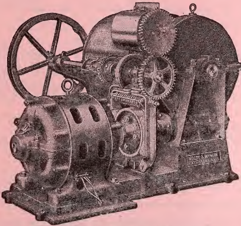
ELECTRIC ELEVATOR MACHINE
